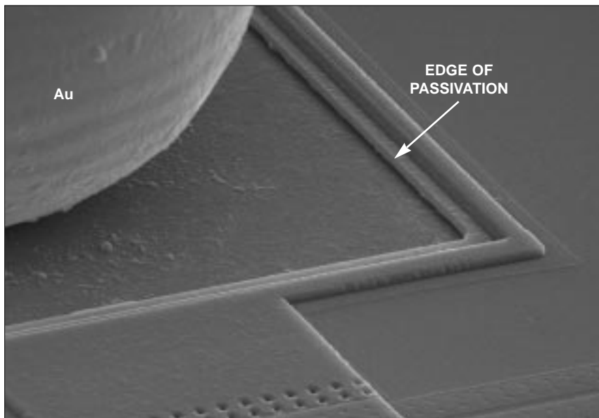
Figure 4. SEM views of typical wirebonding. 60°.
