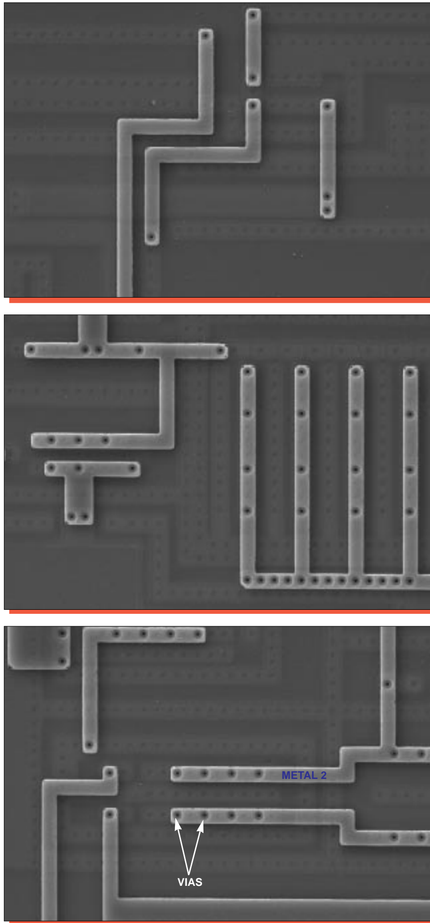
Figure 13. Topological SEM views of metal 2 patterning. Mag. 1600x, 0°.
