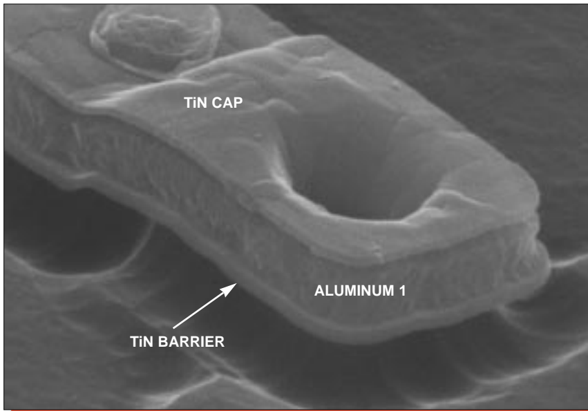
Figure 19. Perspective SEM views of metal 1 step coverage. 60°.
