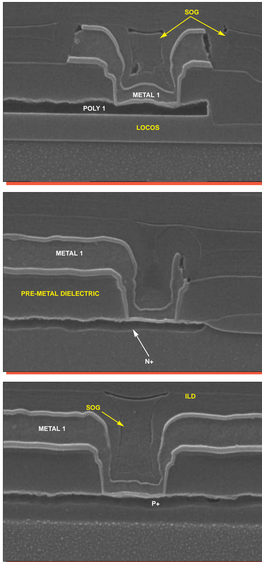
Figure 20. SEM section views of typical metal 1 contacts. Mag. 26,000x.
