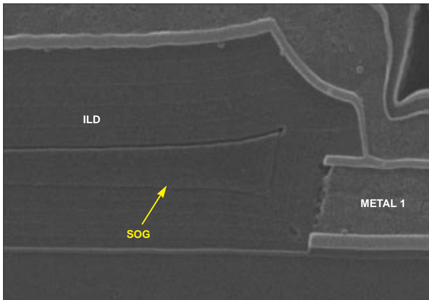
Figure 15. SEM section views illustrating typical vias and interlevel dielectric composition.
