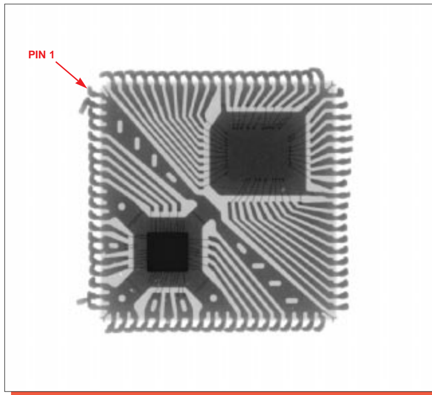
Figure 2. X-ray view of the package. Mag. 4.5x.
