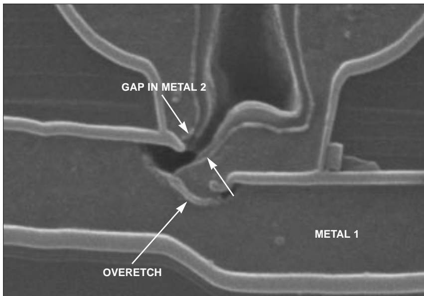
Figure 16. SEM section views of via defects.
