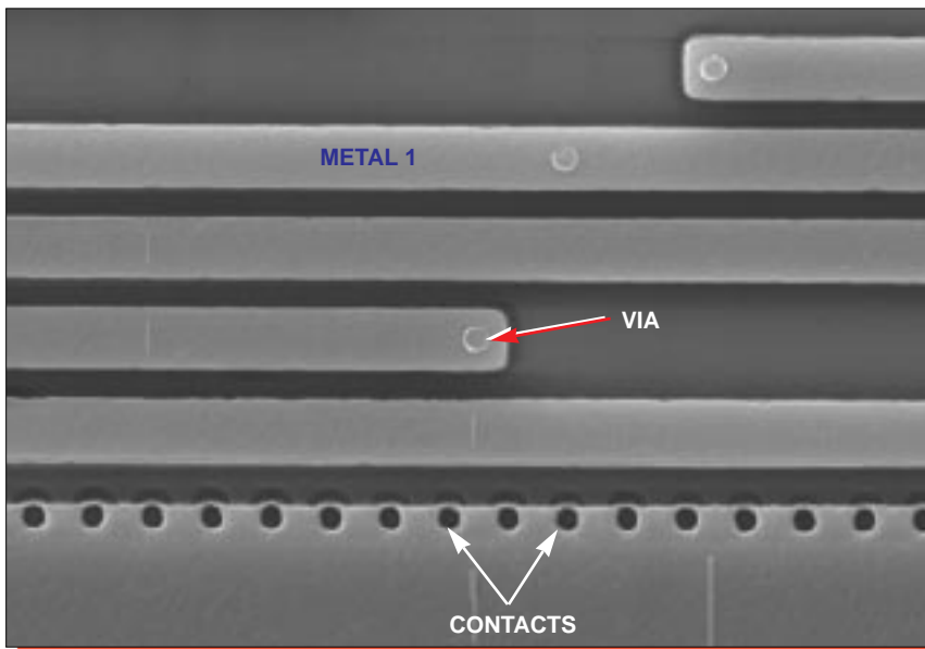
Figure 18. Topological SEM views of metal 1 patterning. 0°.
