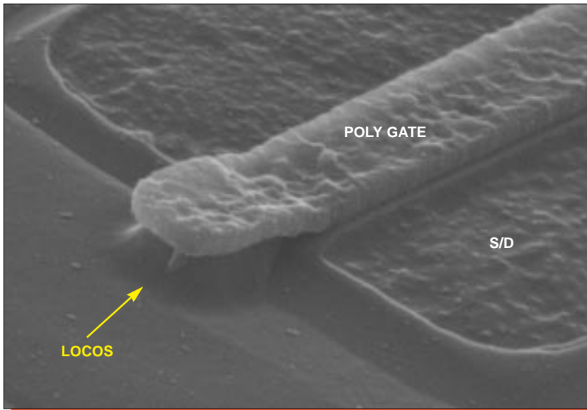
Figure 23. Perspective SEM views of poly coverage. 60°.
