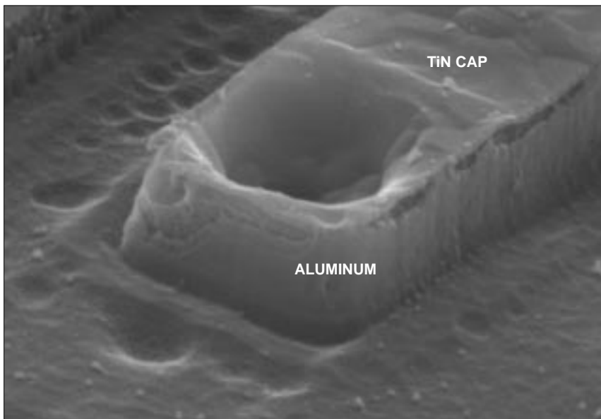
Figure 14. Perspective SEM views of metal 2 step coverage. 60°.
