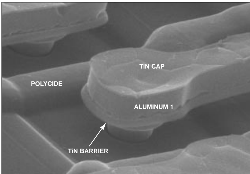
Figure 20. Perspective SEM views of metal 1 step coverage. 60°.
