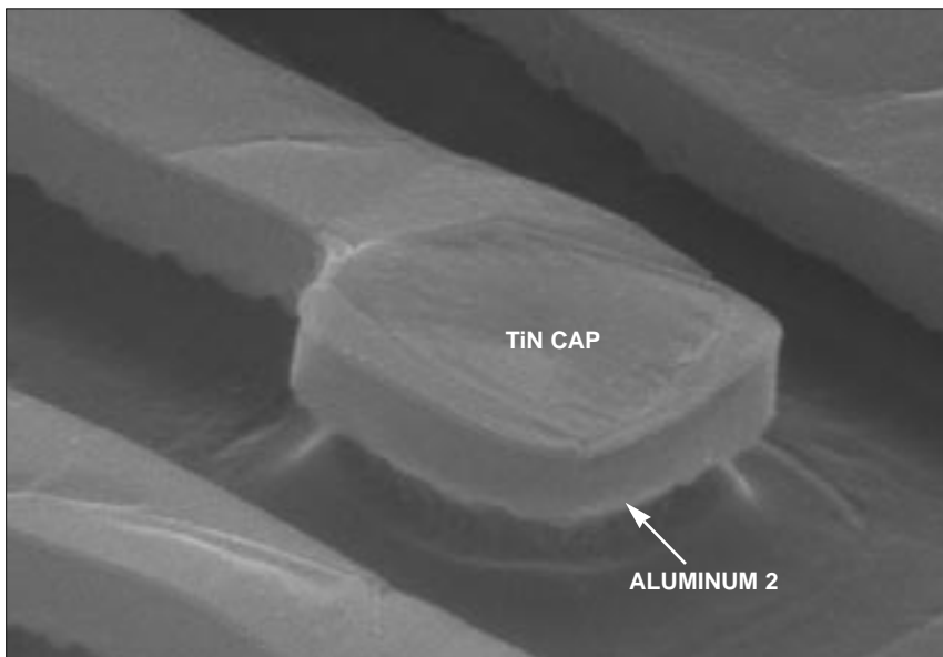
Figure 16. Perspective SEM views of metal 2 step coverage. 60°.
