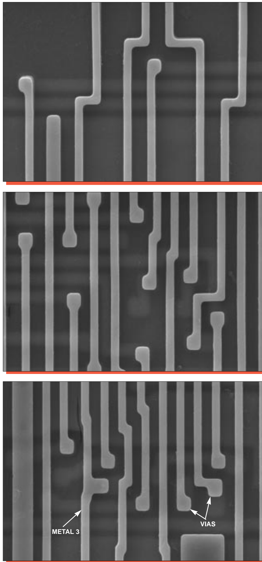
Figure 11. Topological SEM views of metal 3 patterning. Mag. 3200x, 0°.
