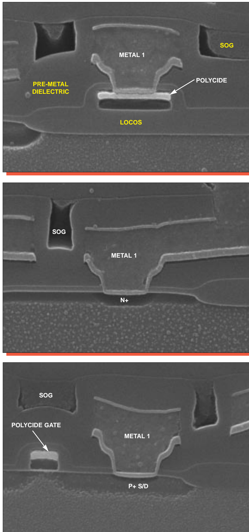
Figure 21. SEM section views of typical metal 1 contacts. Mag. 26,000x.
