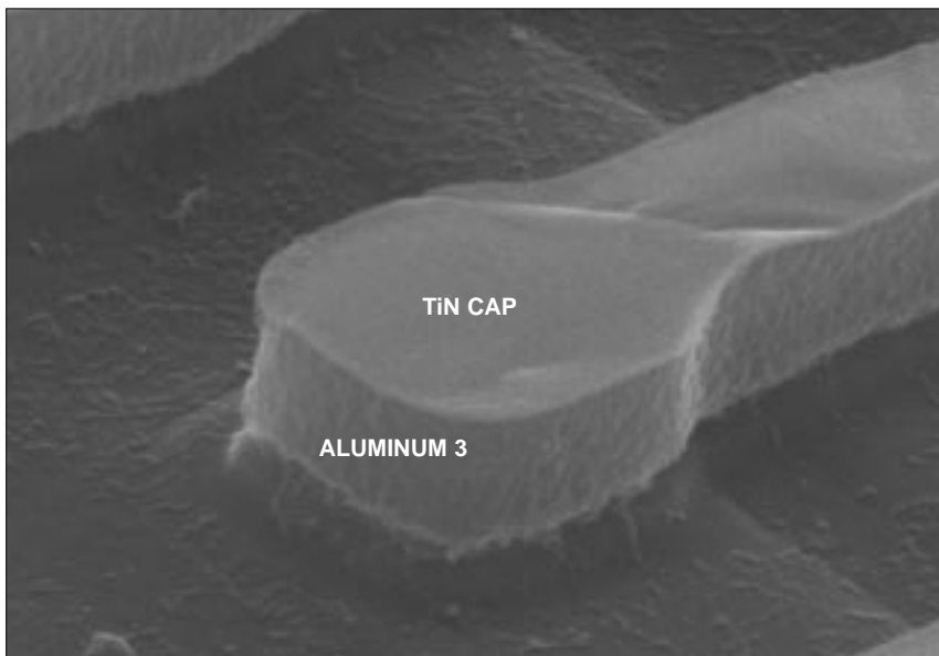
Figure 12. Perspective SEM views of metal 3 step coverage. 60°.
