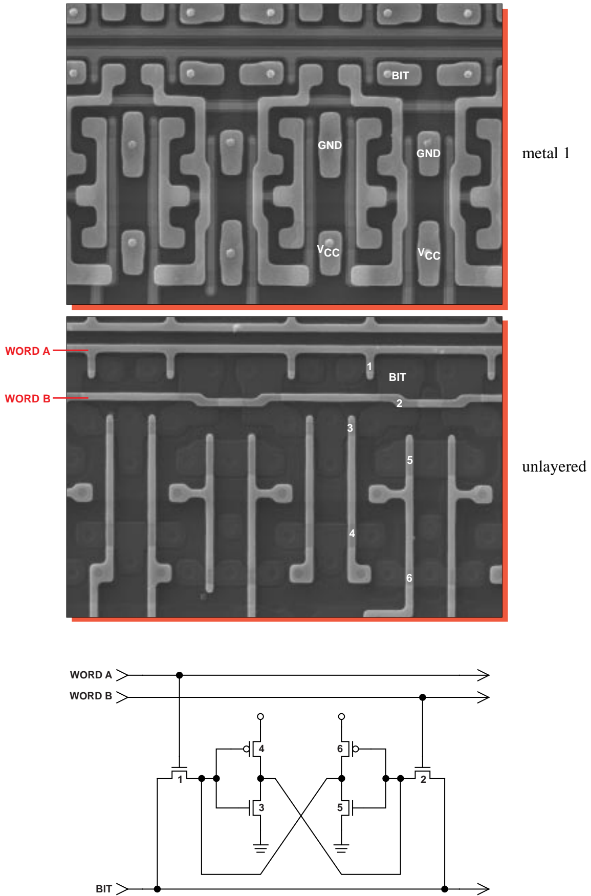
Figure 31. Topological SEM views and schematic of the FPGA Base 6T-SRAM cell. Mag. 3200x.
