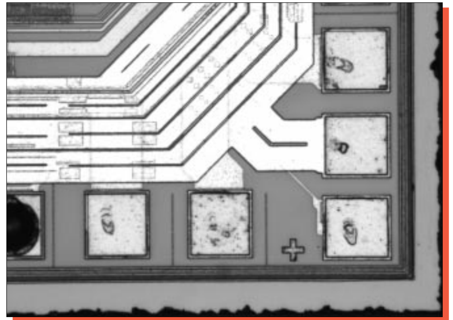
Figure 6. Optical views of die corners. Mag. 170x.
