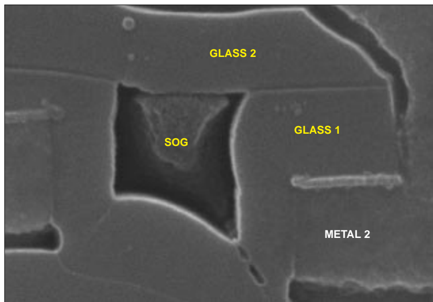
Figure 13. SEM section views illustrating a typical M3-to-M2 via and interlevel dielectric 2 composition.
