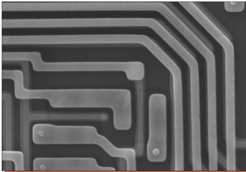
Figure 19. Topological SEM views of metal 1 patterning. 0°.
