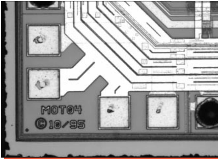
Figure 6. Optical views of die corners. Mag. 170x.
