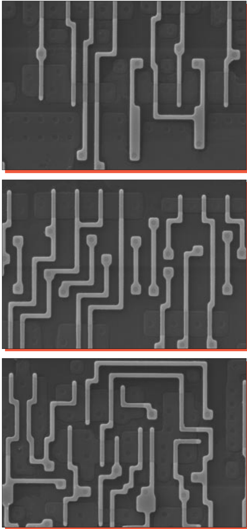
Figure 22. Topological SEM views of polycide patterning. Mag. 3200x, 0°.
