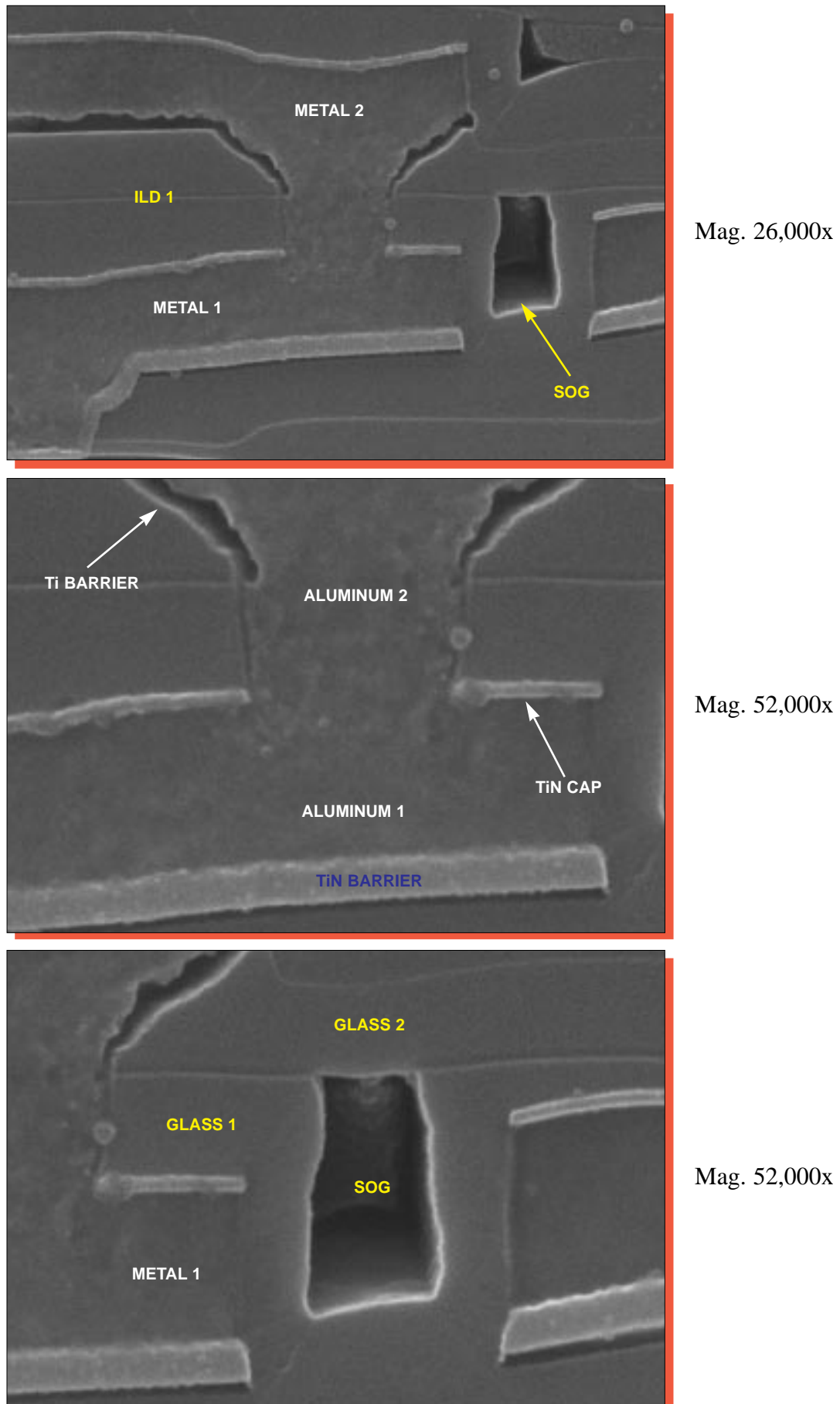
Figure 17. SEM section views illustrating a typical M2-to-M1 via and interlevel dielectric 1 composition.
