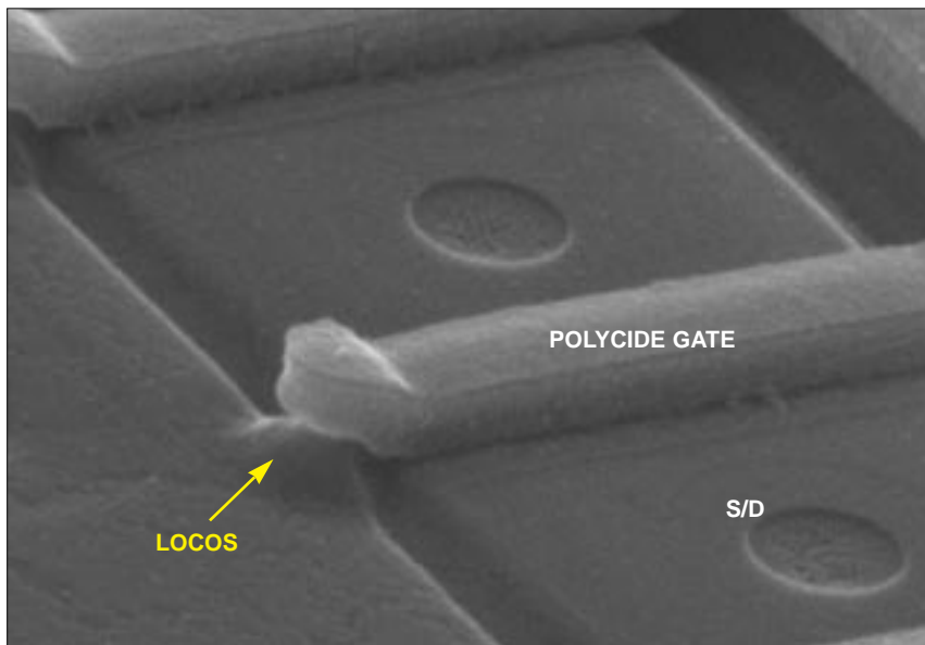
Figure 23. Perspective SEM views of polycide coverage. 60°.
