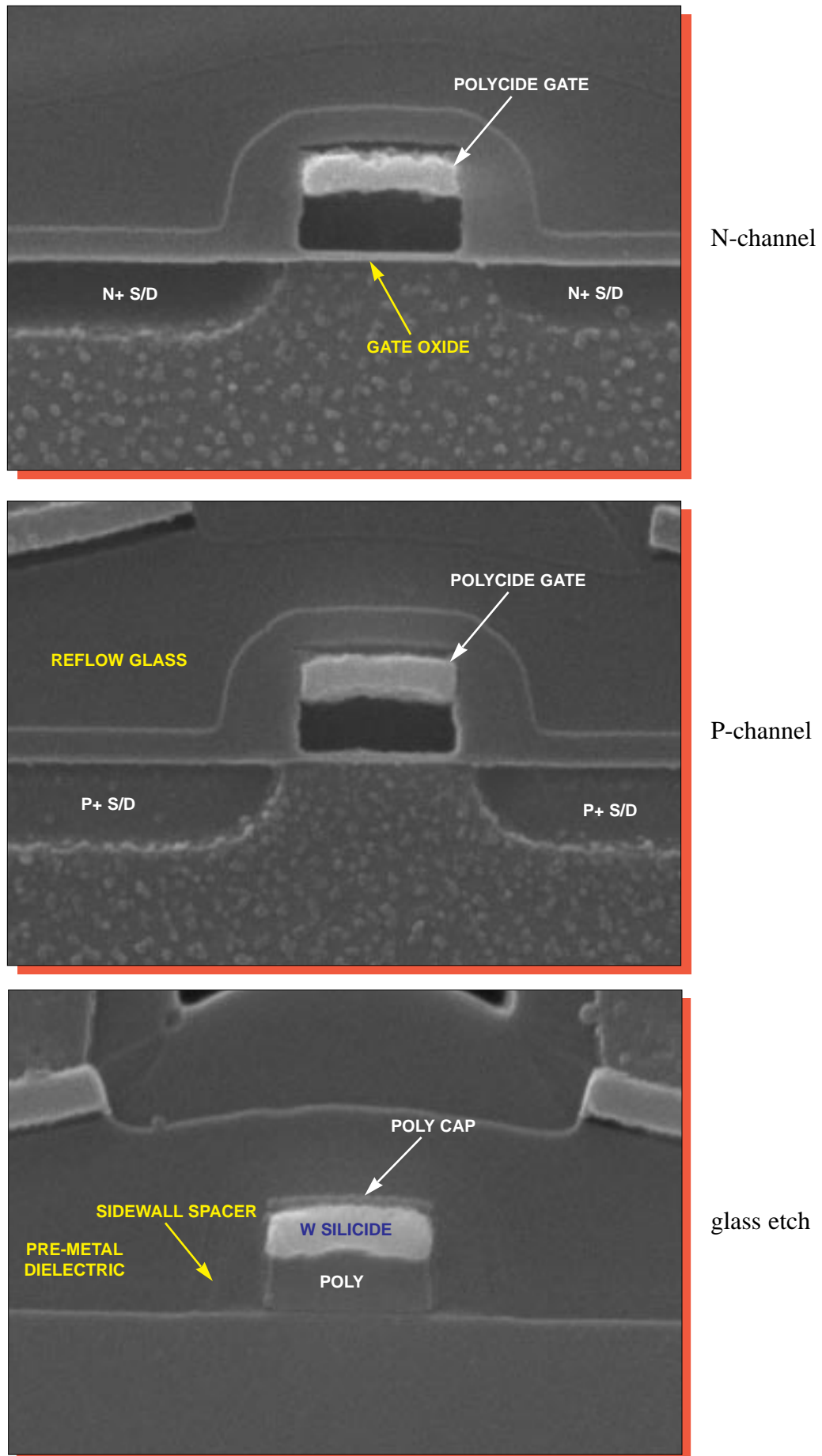
Figure 24. SEM section views of typical transistors. Mag. 52,000x.
